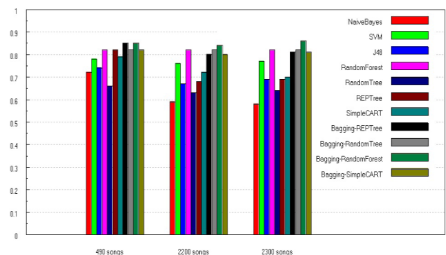
Figure 2: Recall statistics
