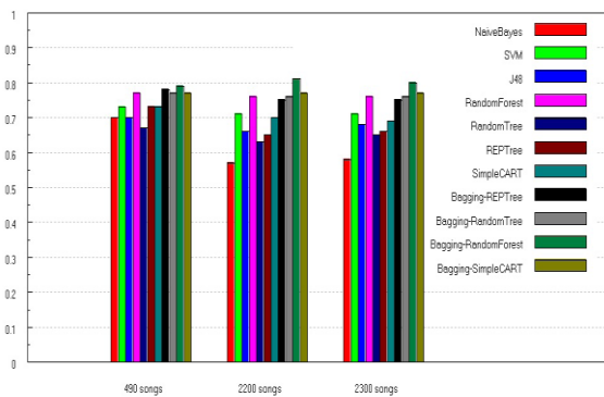
Figure 4: F-measure statistics
