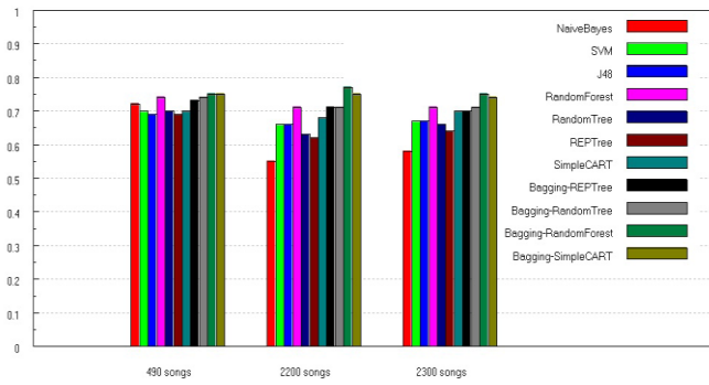
Figure 3: Precision statistics
