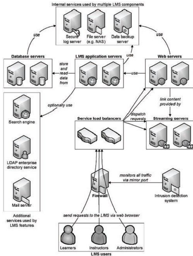
Fig. 5 Components Of A Typical Learning Management System Infrastructure
