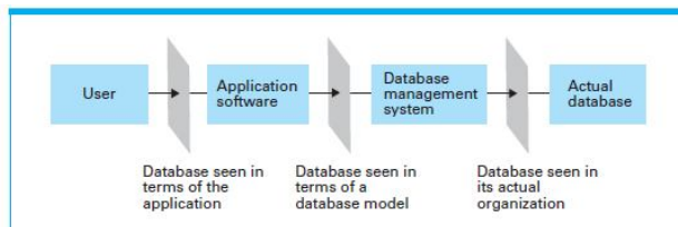
Fig. 2 The conceptual layers of a database management
