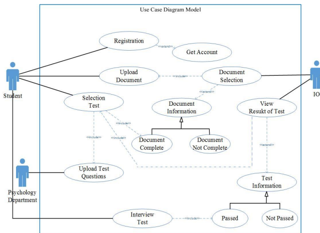
Fig. 9 Use Case Diagram Model
