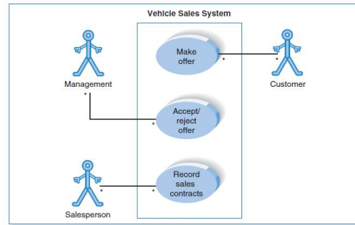
Fig. 7 Use Case Diagram for Vehicle Sales System
