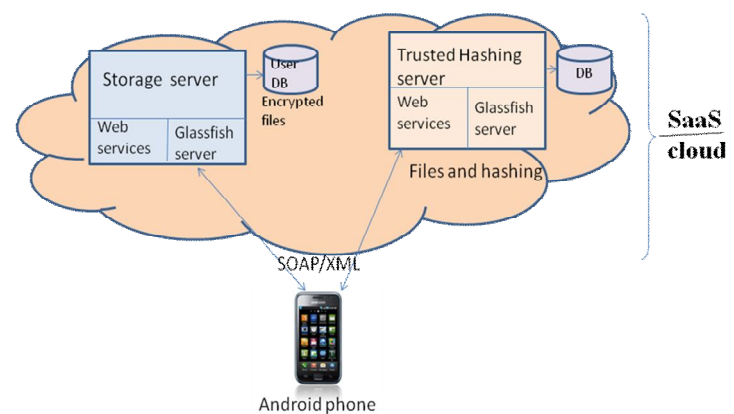
Fig 2: system architecture.
