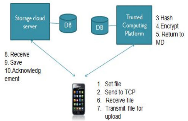
Fig. 3 steps in uploading process
